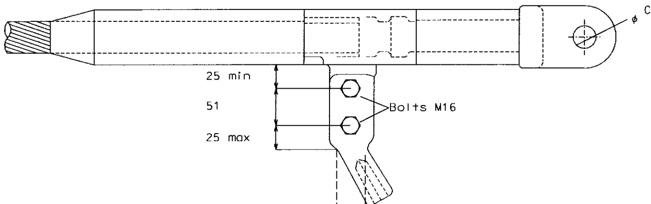
Straight Jumper Terminal Type 2
