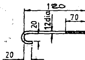
DETAIL OF J BOLT
