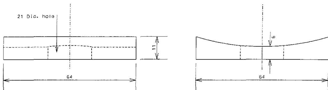
DETAIL 64 X 64 CURVED WASHER
