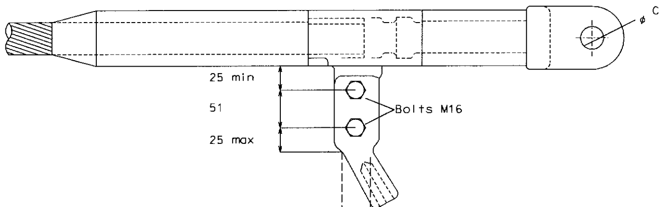
Straight Jumper Terminal Type 5 only
