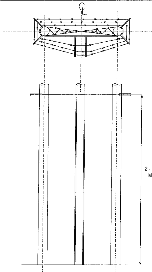
GENERAL ARRANGEMENT.
