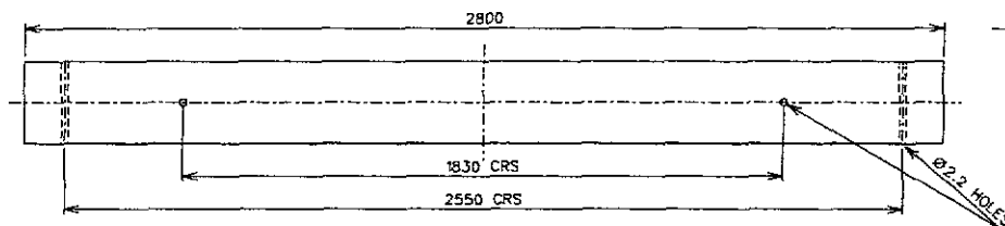
TYPE M.441/3 6ft H-POLE LOWER BAULK BOG SHOE
