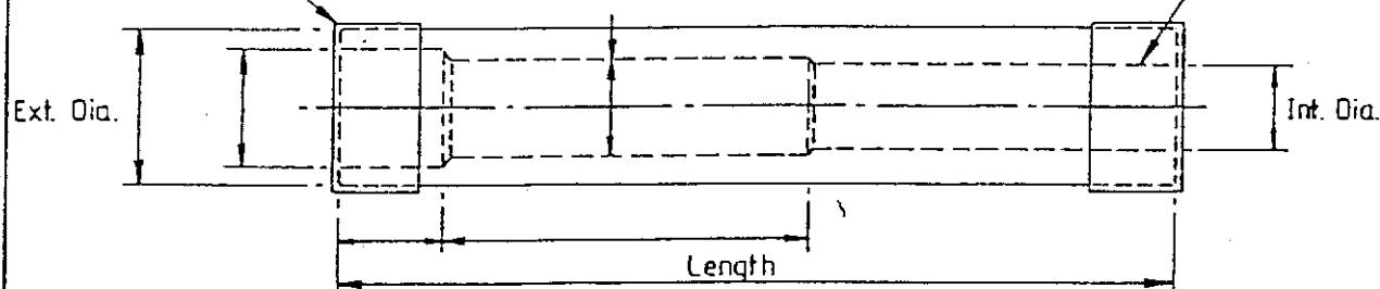
FIG II
