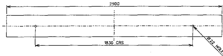
TYPE M.441/2 6' H-POLE LOWER BAULK NO BOG SHOE
