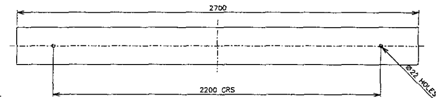
TYPE M.441/4 6ft H-POLE ≤ 14m DIAGONAL BRACE
