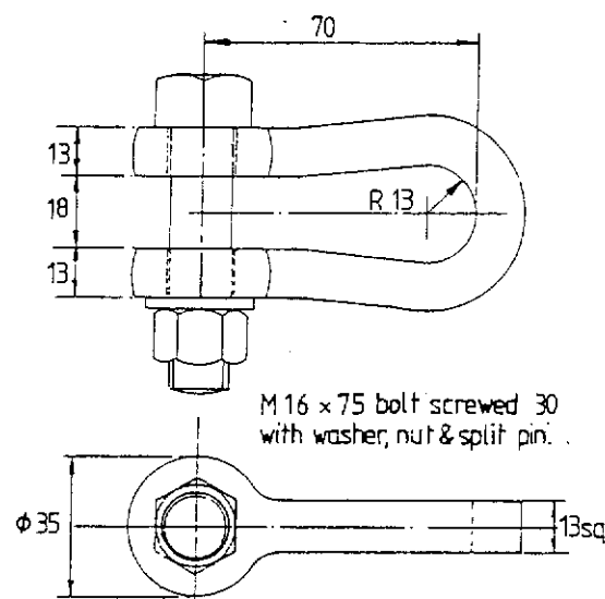
TYPE M 1/3
