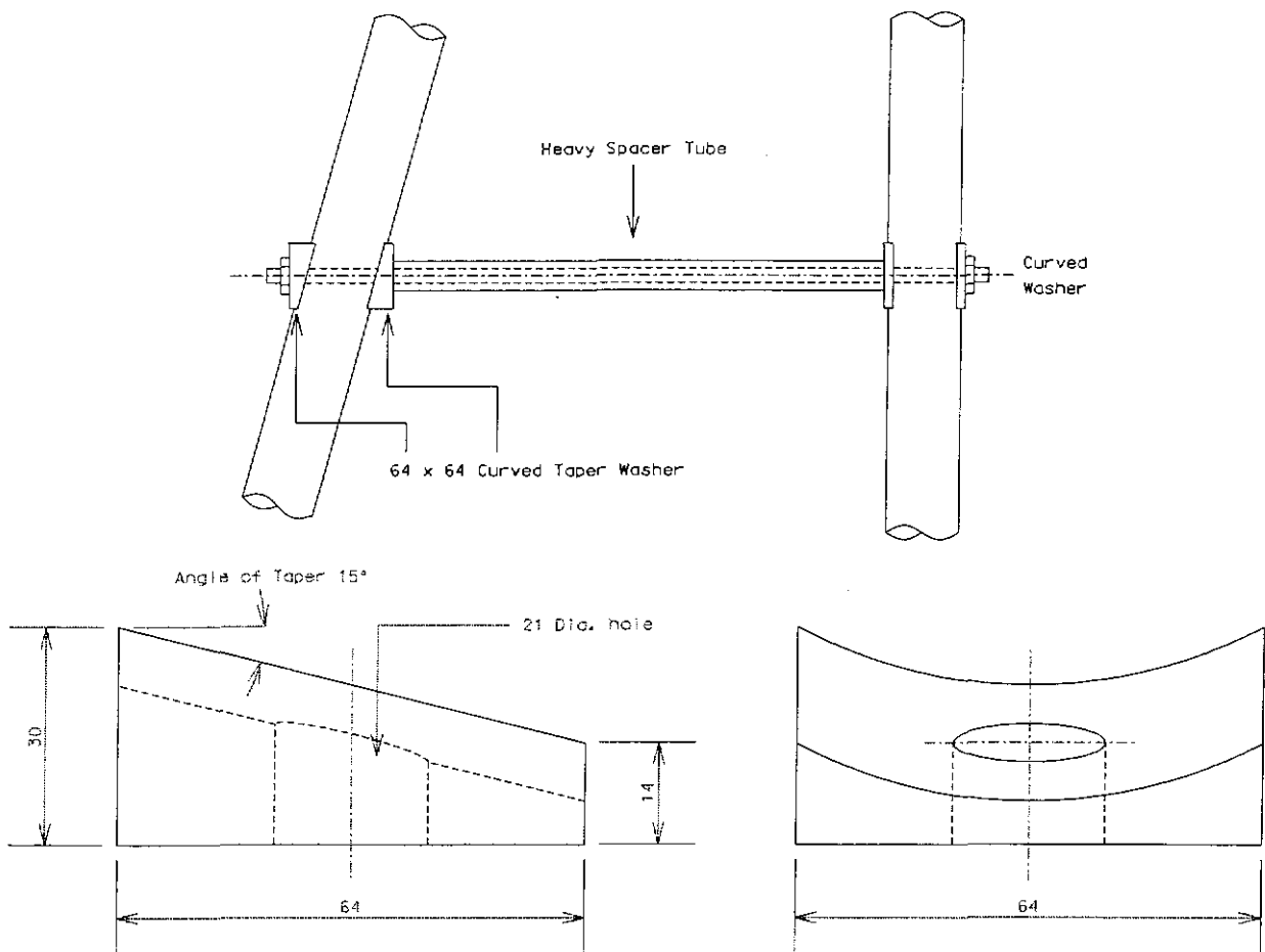
DETAIL 64 X 64 CURVED TAPER WASHER
