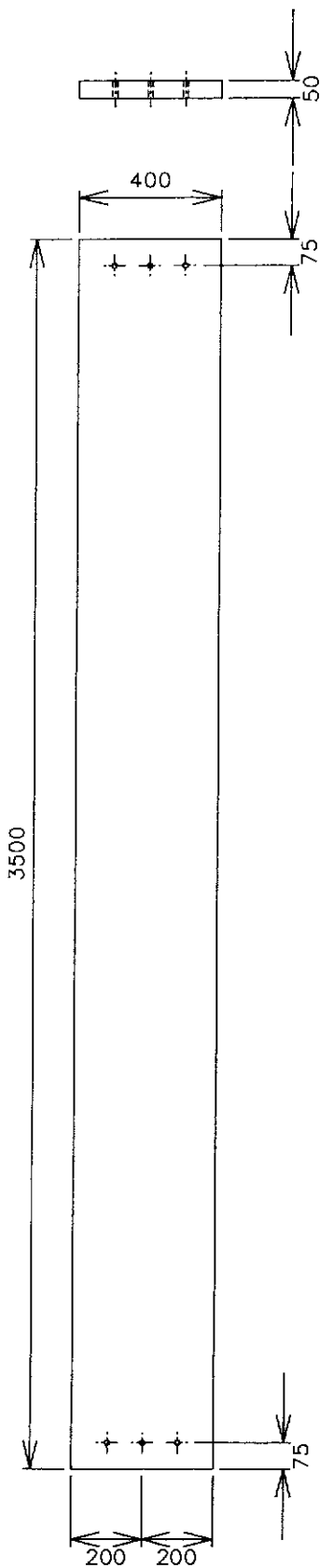
MIN No 176/1
