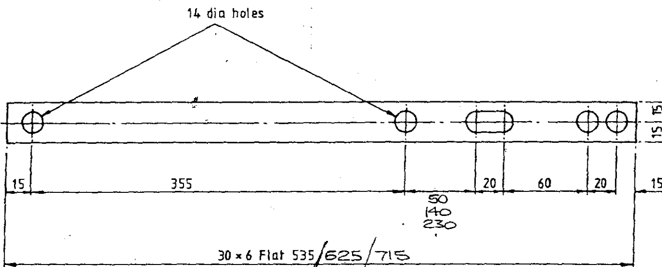
DETAIL OF SUPPORTING STRAP
