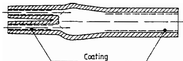
TYPE 2.
