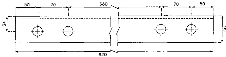
ITEM 1 60x60x6 BSEA
