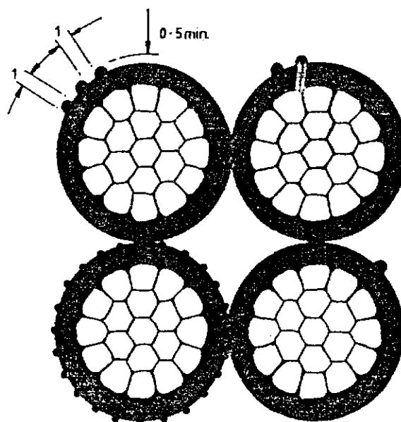
Sequence and Dimensions of Phase Identification Ribs
