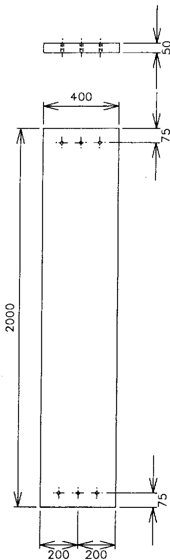
MIN No 176/2
