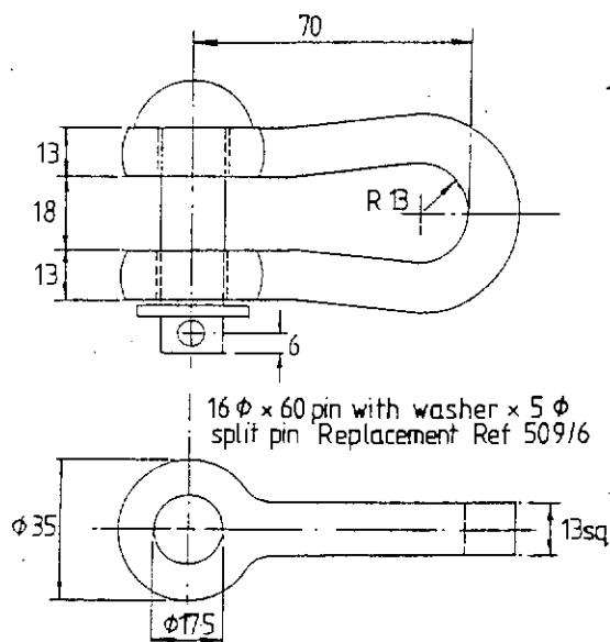
TYPE M 1/2
