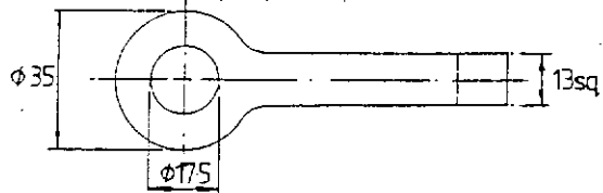
TYPE M 1/2
