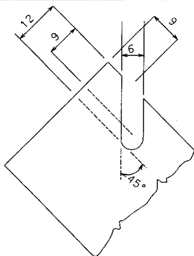
METHOD OF FIXING BARBED WIRE TO OUTRIGGER BKT.
