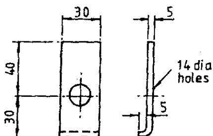
DETAIL OF FIXING CLIP
